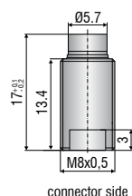
connector side
