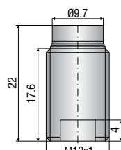
connector side
