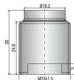
connector side
