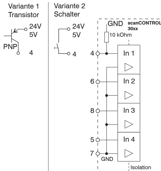
Abb. 27 Pull-down
