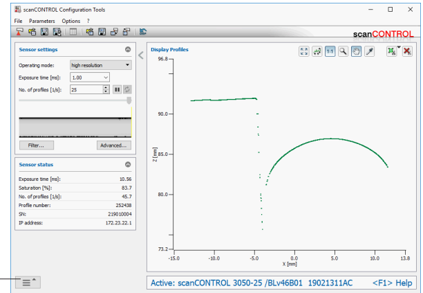
Abb. 36 Screenshot scanCONTROL Configuration Tools
