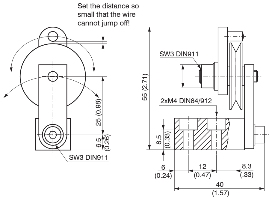
Fig. 11 Deflection pulley TR1-WDS with mounting foot, dimensions in mm (inches, rounded off)
