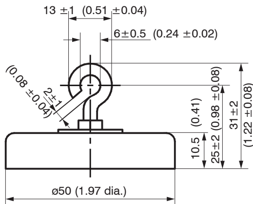
Fig. 10 Magnetic holder MH1 - WDS, dimensions in mm (inches, rounded off)
