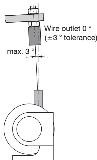
Fig. 8 Attachment and maximum diagonal pull of the measuring wire
