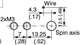
Fig. 7 Drilling pattern WDS - ... - MPM, dimensions in mm (inches, rounded off)
