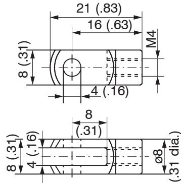
Fig. 14 Fork head with folding spring bolt GK1-WDS, dimensions in mm (inches, rounded off)
