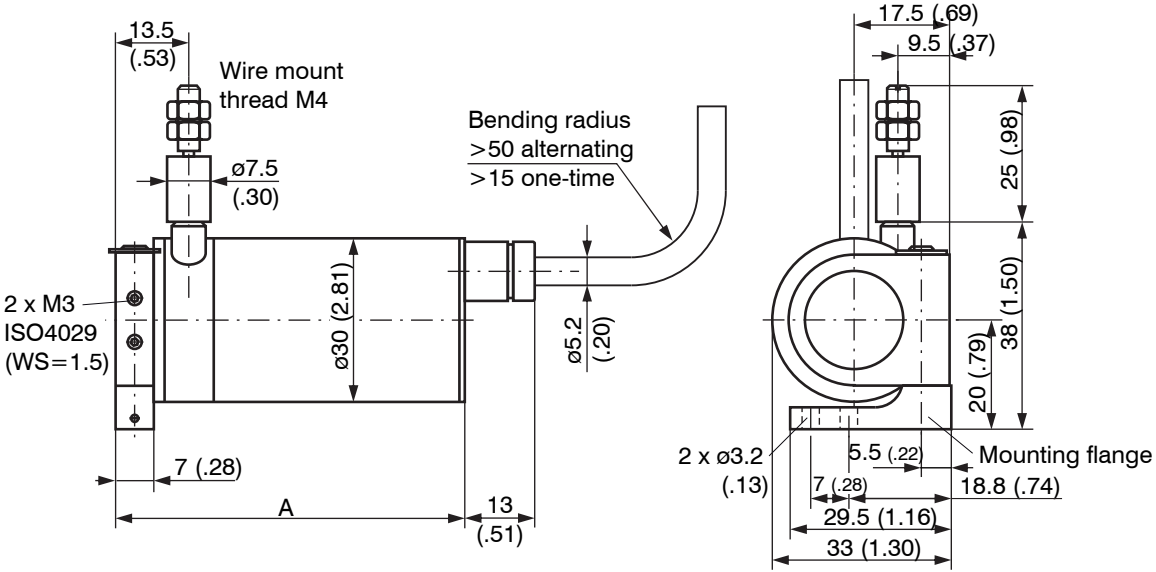
Fig. 6 Dimensional drawing WDS - ... - MPM, dimensions in mm, (inches, rounded off)
