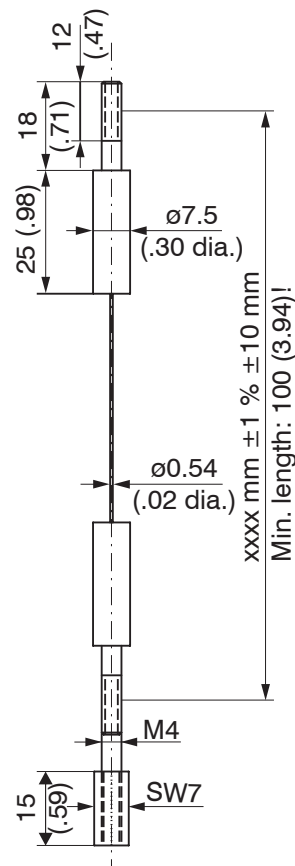
Fig. 13 Wire extension WE-xxxx-M4
