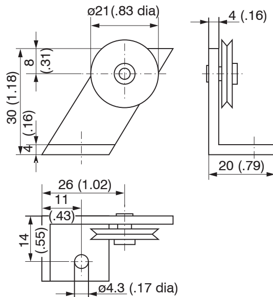
Fig. 12 Deflection pulley TR3-WDS, fixed, with mounting foot
