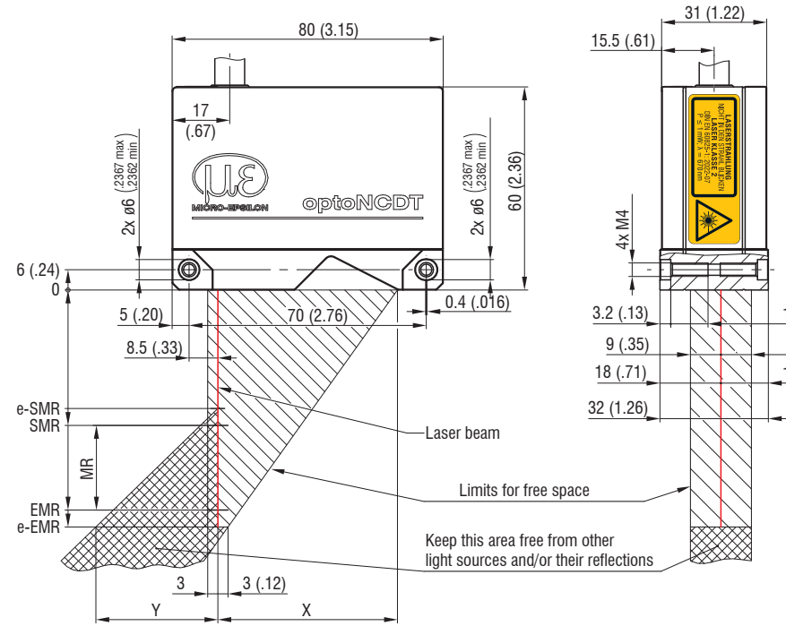
Dimensional drawing ILD5500-10/25/50 dimensions in mm (inches)
