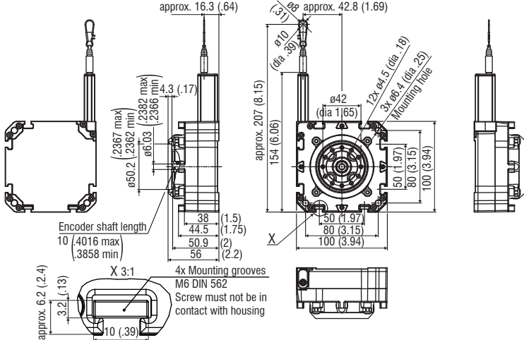
Dimensional drawing of WPS-3500-K100-M / WPS-5000-K100-M / WPS-8000-K100-M, dimensions in mm (inches, rounded off)
