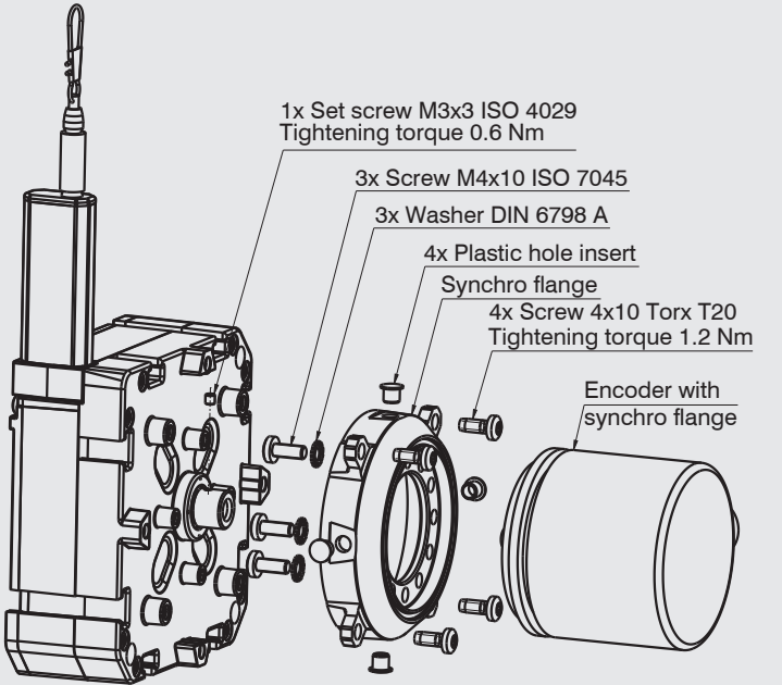
Mounting the synchro flange adapter and encoder, WPS-3500-K100-M / WPS-5000-K100-M / WPS-8000-K100-M
