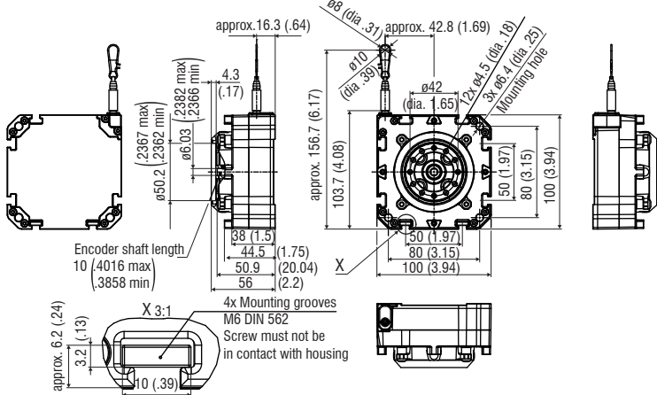
Dimensional drawing of WPS-1500-K100-M / WPS-2500-K100-M, dimensions in mm (inches, rounded off)
