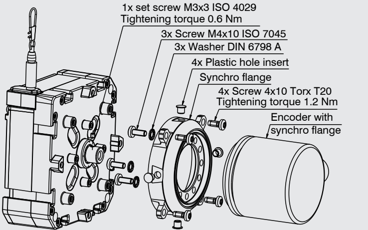
Mounting the synchro flange adapter and encoder, WPS-1500-K100-M / WPS-2500-K100-M
