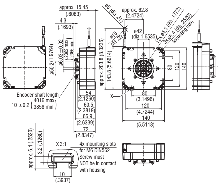
Dimensional drawing of WPS-12000-K140-M dimensions in mm (inches, rounded off)
