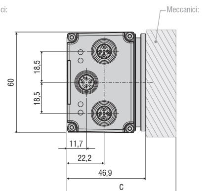
Uscita PN/ENIP/CAT
